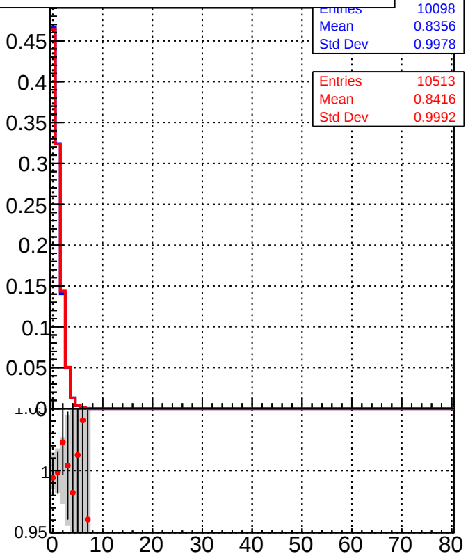
Legend: /data2/legianni/BDT-vs-DNN/real-BDT/CMSSW_13_0_0_pre4/src/runrem/DQM_TT_mkFit_ (blue line with squares), DQM_TT_mkFitRETEST2_ (red line with circles)
