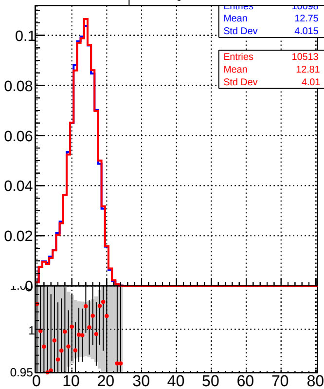
Legend: /data2/legianni/BDT-vs-DNN/real-BDT/CMSSW_13_0_0_pre4/src/runrem/DQM_TT_mkFit_ (blue line with squares), DQM_TT_mkFitRETEST2_ (red line with circles)
