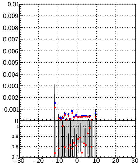
/data2/legianni/BDT-vs-DNN/real-BDT/CMSSW_13_0_0_pre4/src/runrem/DQM_TT_mkFit_ Fake rate vs d DQM_TT_mkFitRETEST2
