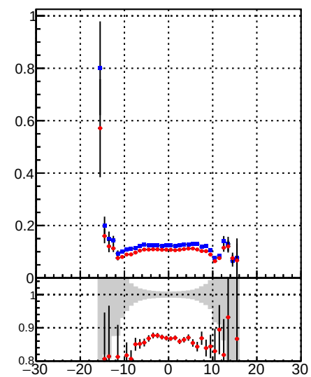
/data2/legianni/BDT-vs-DNN/real-BDT/CMSSW_13_0_0_pre4/src/runrem/DQM_TT_mkFit_ Fake rate vs d DQM_TT_mkFitRETEST2
