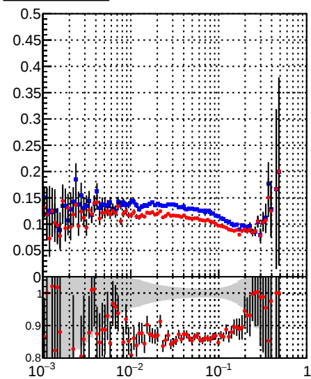
—•— /data2/legianni/BDT-vs-DNN/real-BDT/CMSSW_13_0_0_pre4/src/runrem/DQM_TT_mkFit_ —•— DQM_TT_mkFitRETEST2_
