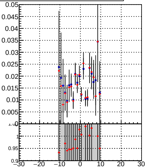
Efficiency vs vertpos - /data2/legianni/BDT-vs-DNN/real-BDT/CMSSW_13_0_0_pre4/src/runrem/DQM_TT_mkFit_ - DQM_TT_mkFitRETEST2_
