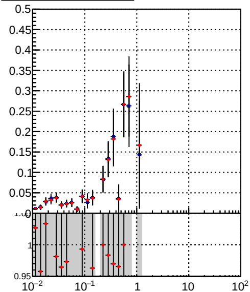
Efficiency vs vertpos - /data2/legianni/BDT-vs-DNN/real-BDT/CMSSW_13_0_0_pre4/src/runrem/DQM_TT_mkFit_ - DQM_TT_mkFitRETEST2_
