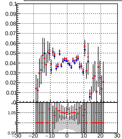
Efficiency vs vertpos - /data2/legianni/BDT-vs-DNN/real-BDT/CMSSW_13_0_0_pre4/src/runrem/DQM_TT_mkFit_ - DQM_TT_mkFitRETEST2_
