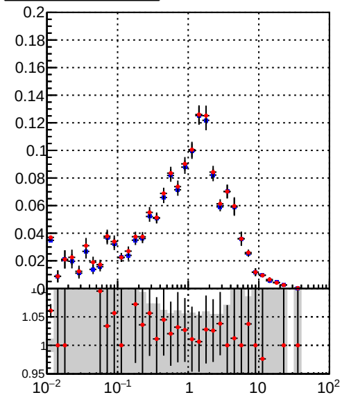
Efficiency vs vertpos - /data2/legianni/BDT-vs-DNN/real-BDT/CMSSW_13_0_0_pre4/src/runrem/DQM_TT_mkFit_ - DQM_TT_mkFitRETEST2_
