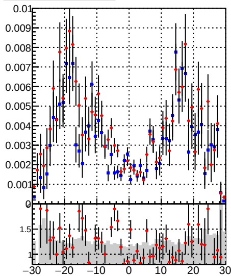
Fake rate vs d —•— /data2/legianni/BDT-vs-DNN/real-BDT/CMSSW_13_0_0_pre4/src/runrem/DQM_TT_mkFit_ —•— DQM_TT_mkFitRETEST2
