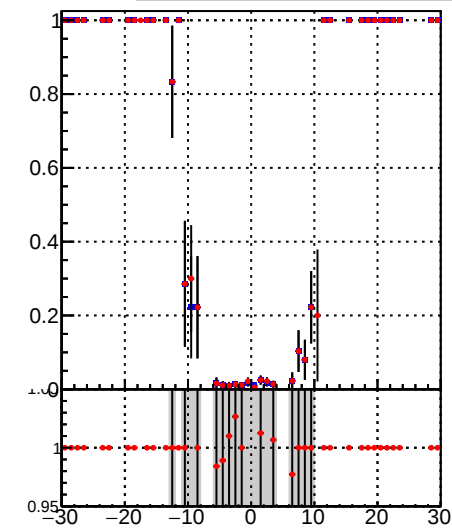
Fake rate vs v ■ /data2/legianni/BDT-vs-DNN/real-BDT/CMSSW_13_0_0_pre4/src/runrem/DQM_TT_mkFit_ ● DQM_TT_mkFitRETEST2_
