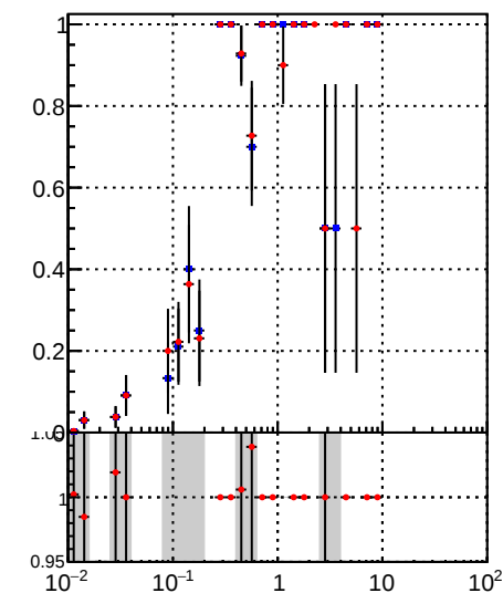
Fake rate vs v ■ /data2/legianni/BDT-vs-DNN/real-BDT/CMSSW_13_0_0_pre4/src/runrem/DQM_TT_mkFit_ ● DQM_TT_mkFitRETEST2_
