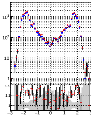
N of reco track vs \eta /data2/legianni/BDT-vs-DNN/real-BDT/CMSSW_13_0_0_pre4/src/runrem/DQM_TT_mkFit DQM_TT_mkFitRETEST2 ps eta
