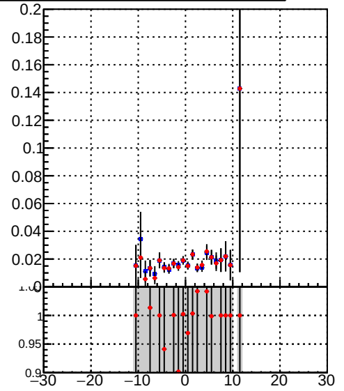
— /data2/legianni/BDT-vs-DNN/real-BDT/CMSSW_13_0_0_pre4/src/runrem/DQM_TT_mkFit_ — DQM_TT_mkFitRETEST2_
