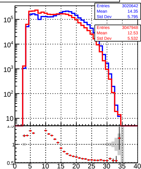
mean hit — /data2/legianni/BDT-vs-DNN/real-BDT/CMSSW_13_0_0_pre4/src/runrem/DQM_TT_mkFit_ — DQM_TT_mkFitRETEST2_
