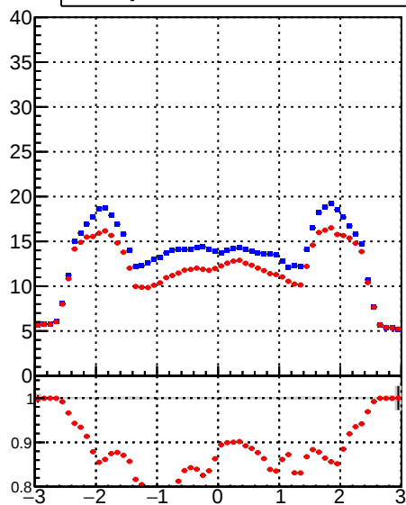
mean hit — /data2/legianni/BDT-vs-DNN/real-BDT/CMSSW_13_0_0_pre4/src/runrem/DQM_TT_mkFit_ — DQM_TT_mkFitRETEST2_
