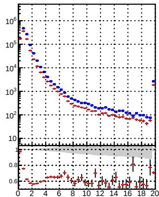
N of reco track vs. \chi^2 \frac{\text{DQM\_TT\_mkFitRETEST2}}{\text{DQM\_TT\_mkFit}}
