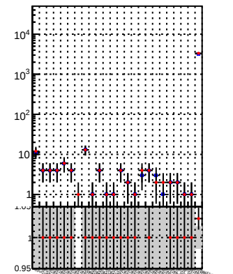
N of reco track vs. \chi^2 - /data2/legianni/BDT-vs-DNN/real-BDT/CMSSW_13_0_0_pre4/src/runrem/DQM_TT_mkFit_ - DQM_TT_mkFitRETEST2_
