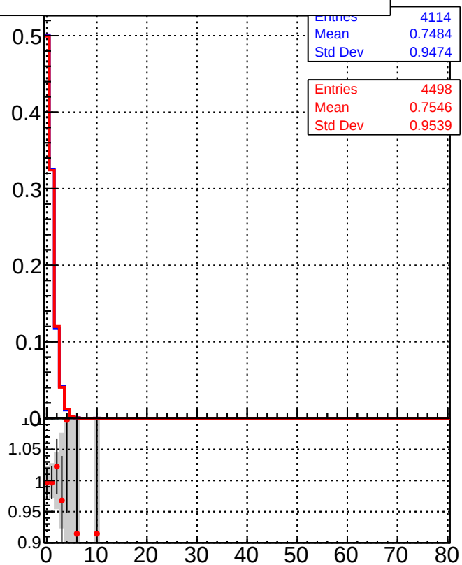
Legend for the bottom row plots: █ — ■ /data2/legianni/BDT-vs-DNN/real-BDT/CMSSW_13_0_0_pre4/src/runrem/DQM_TT_mkFit_ — ● DQM_TT_mkFitRETEST2_
