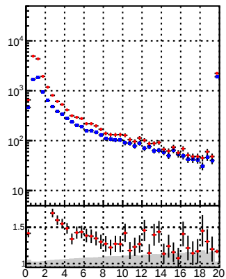
N of reco track vs. \chi^2 Legend: \bullet /data2/legianni/BDT-vs-DNN/real-BDT/CMSSW_13_0_0_pre4/src/runrem/DQM_TT_mkFit \bullet DQM_TT_mkFitRETEST2
