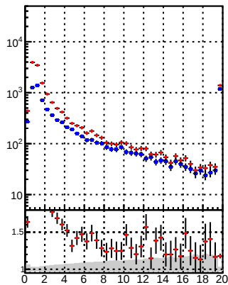
N of reco track vs. \chi^2 Legend: \bullet /data2/legianni/BDT-vs-DNN/real-BDT/CMSSW_13_0_0_pre4/src/runrem/DQM_TT_mkFit \bullet DQM_TT_mkFitRETEST2
