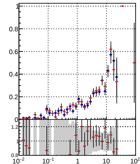
—■— /data2/legianni/BDT-vs-DNN/real-BDT/CMSSW_13_0_0_pre4/src/runrem/DQM_TT_mkFit_ —●— DQM_TT_mkFitRETEST2_ Fake rate vs v
