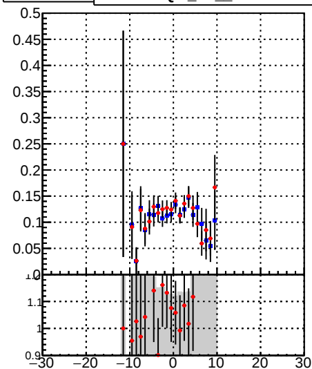
—■— /data2/legianni/BDT-vs-DNN/real-BDT/CMSSW_13_0_0_pre4/src/runrem/DQM_TT_mkFit_ —●— DQM_TT_mkFitRETEST2_ Fake rate vs v
