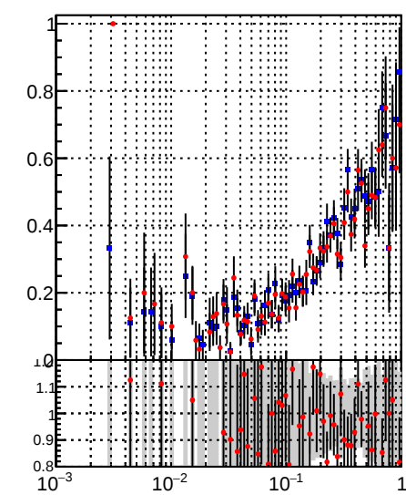
Legend: /data2/legianni/BDT-vs-DNN/real-BDT/CMSSW_13_0_0_pre4/src/runrem/DQM_TT_mkFit_ (blue line with dots), DQM_TT_mkFitRETEST2_ (red line with dots)
