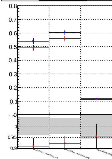
Fake rate vs. - /data2/legianni/BDT-vs-DNN/real-BDT/CMSSW_13_0_0_pre4/src/runrem/DQM_TT_mkFit_ - DQM_TT_mkFitRETEST2_
