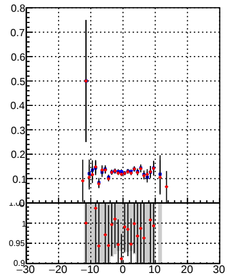
/data2/legianni/BDT-vs-DNN/real-BDT/CMSSW_13_0_0_pre4/src/runrem/DQM_TT_mkFit_ DQM_TT_mkFitRETEST2
