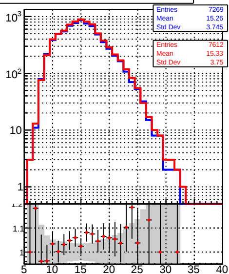
/data2/legianni/BDT-vs-DNN/real-BDT/CMSSW_13_0_0_pre4/src/runrem/DQM_TT_mkFit_ DQM_TT_mkFitRETEST2_
