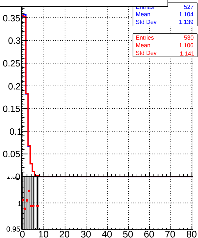
/data2/legianni/BDT-vs-DNN/real-BDT/CMSSW_13_0_0_pre4/src/runrem/DQM_TT_mkFit_ DQM_TT_mkFitRETEST2_
