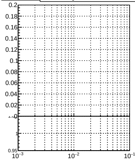
—●— /data2/legianni/BDT-vs-DNN/real-BDT/CMSSW_13_0_0_pre4/src/runrem/DQM_TT_mkFit_ —●— DQM_TT_mkFitRETEST2_
