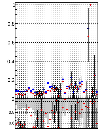
Fake rate vs. —●— /data2/legianni/BDT-vs-DNN/real-BDT/CMSSW_13_0_0_pre4/src/runrem/DQM_TT_mkFit_ —●— DQM_TT_mkFitRETEST2
