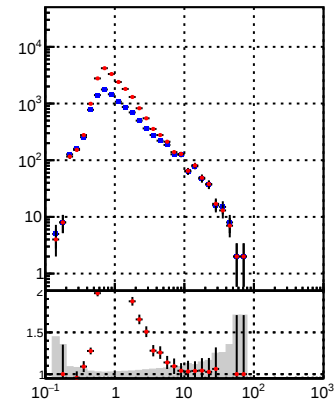
/data2/legianni/BDT-vs-DNN/real-BDT/CMSSW_13_0_0_pre4/src/runrem/DQM_TT_mkFit DQM_TT_mkFitRETEST2
