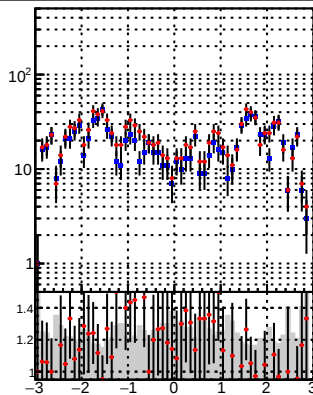
/data2/legianni/BDT-vs-DNN/real-BDT/CMSSW_13_0_0_pre4/src/runrem/DQM_TT_mkFit DQM_TT_mkFitRETEST2
