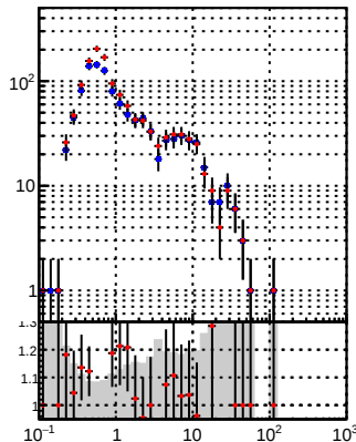
/data2/legianni/BDT-vs-DNN/real-BDT/CMSSW_13_0_0_pre4/src/runrem/DQM_TT_mkFit DQM_TT_mkFitRETEST2
