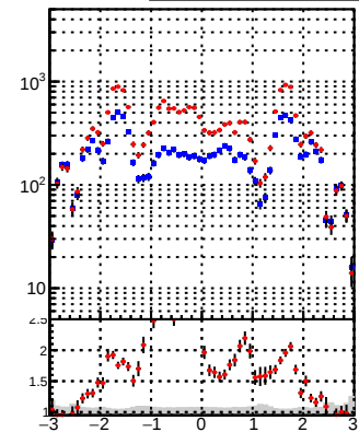
/data2/legianni/BDT-vs-DNN/real-BDT/CMSSW_13_0_0_pre4/src/runrem/DQM_TT_mkFit DQM_TT_mkFitRETEST2
