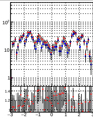
N of reco track vs \eta — /data2/legianni/BDT-vs-DNN/real-BDT/CMSSW_13_0_0_pre4/src/runrem/DQM_TT_mkFit2 — DQM_TT_mkFitRETEST2 \eta eta
