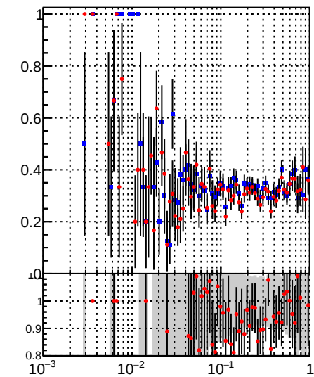
■ /data2/legianni/BDT-vs-DNN/real-BDT/CMSSW_13_0_0_pre4/src/runrem/DQM_TT_mkFit_ ● DQM_TT_mkFitRETEST2_ Fake rate vs
