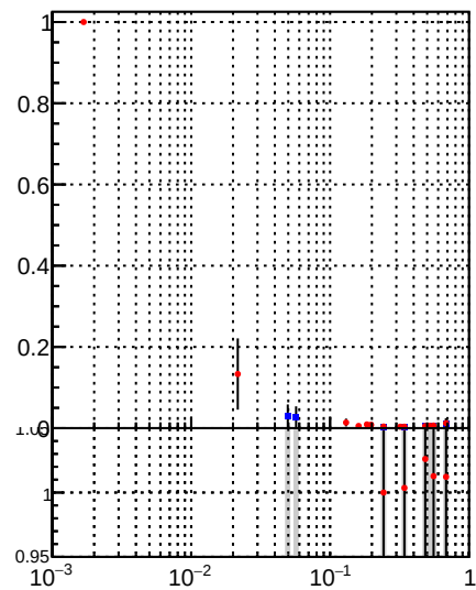
■ /data2/legianni/BDT-vs-DNN/real-BDT/CMSSW_13_0_0_pre4/src/runrem/DQM_TT_mkFit_ ● DQM_TT_mkFitRETEST2_ Duplicates Rate vs dr
