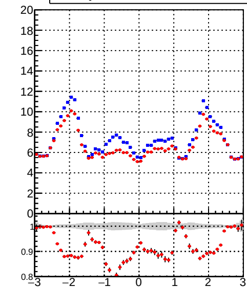
mean hit Legend: — /data2/legianni/BDT-vs-DNN/real-BDT/CMSSW_13_0_0_pre4/src/runrem/DQM_TT_mkFit_ — DQM_TT_mkFitRETEST2_
