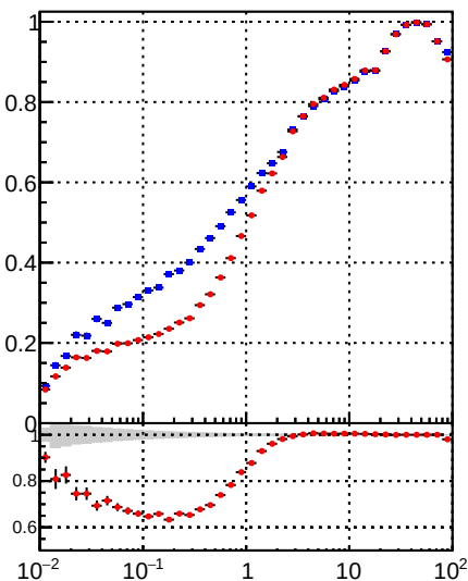
—♦— /data2/legianni/BDT-vs-DNN/real-BDT/CMSSW_13_0_0_pre4/src/runrem/DQM_TT_mkFit_ —•— DQM_TT_mkFitRETEST2_
