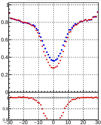
—♦— /data2/legianni/BDT-vs-DNN/real-BDT/CMSSW_13_0_0_pre4/src/runrem/DQM_TT_mkFit_ —•— DQM_TT_mkFitRETEST2_
