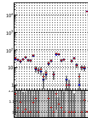
N of reco track vs. \chi^2 \bullet /data2/legianni/BDT-vs-DNN/real-BDT/CMSSW_13_0_0_pre4/src/runrem/DQM_TT_mkFit \bullet DQM_TT_mkFitRETEST2
