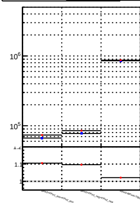
N of reco track vs. \chi^2 verSet
