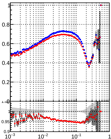
Legend: —•— /data2/legianni/BDT-vs-DNN/real-BDT/CMSSW_13_0_0_pre4/src/runrem/DQM_TT_mkFit_ —•— DQM_TT_mkFitRETEST2_
