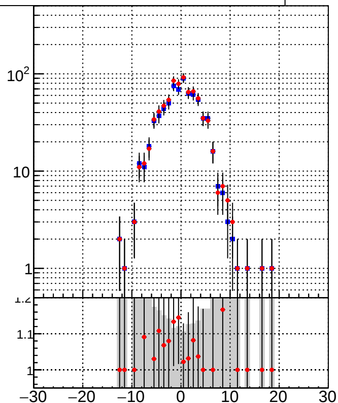
■ /data2/legianni/BDT-vs-DNN/real-BDT/CMSSW_13_0_0_pre4/src/runrem/DQM_TT_mkFit_ ● DQM_TT_mkFitRETEST2_
