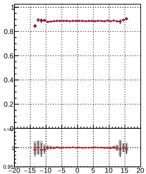
Efficiency vs. \text{sim PV } z
