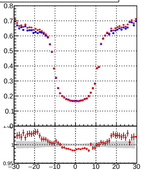
Efficiency vs. \text{sim PV } z Legend: \text{/data2/legianni/BDT-vs-DNN/real-BDT/CMSSW\_13\_0\_0\_pre4/src/runrem/DQM\_TT\_mkFit\_} (Blue line) \text{DQM\_TT\_mkFitRETEST2\_} (Red line)
