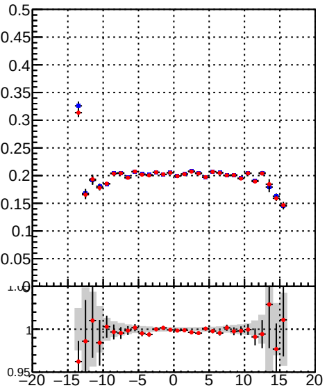
fake+duplicates vs \text{Sim. PV } z
