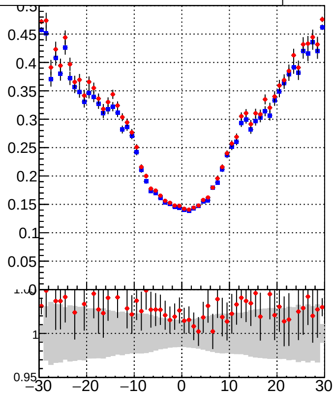
— /data2/legianni/BDT-vs-DNN/real-BDT/CMSSW_13_0_0_pre4/src/runrem/DQM_TT_mkFit_ — DQM_TT_mkFitRETEST2_
