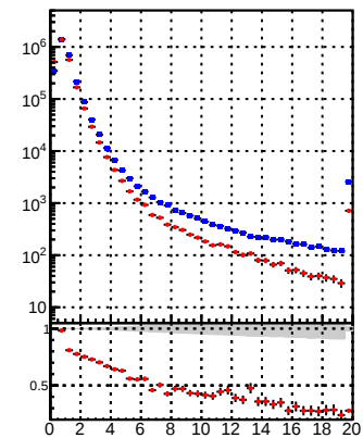
N of reco track vs. \chi^2 for /data2/legianni/BDT-vs-DNN/real-BDT/CMSSW_13_0_0_pre4/src/runrem/DQM_TT_mkFit2
