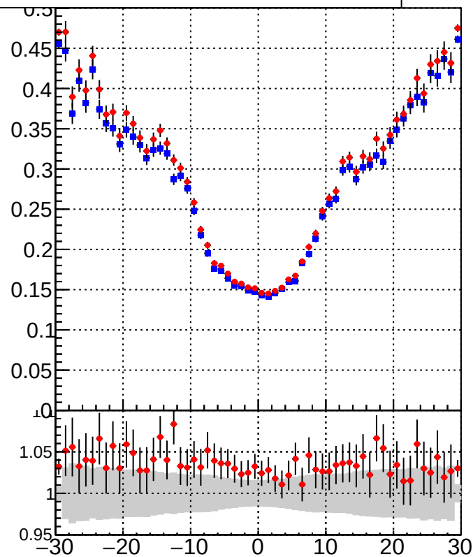
— /data2/legianni/BDT-vs-DNN/real-BDT/CMSSW_13_0_0_pre4/src/runrem/DQM_TT_mkFit_ — DQM_TT_mkFitRETEST2_
