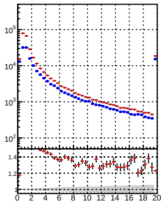
N of reco track vs. \chi^2 for \sqrt{s}=13 TeV, \text{DQM\_TT\_mkFit} vs \text{mkFitRETEST2}
