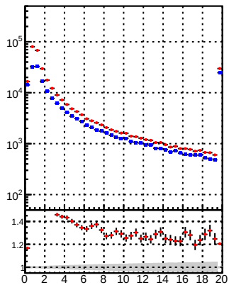
N of reco track vs. \chi^2 for \sqrt{s}=13 TeV, \text{DQM\_TT\_mkFit} vs \text{mkFitRETEST2}
