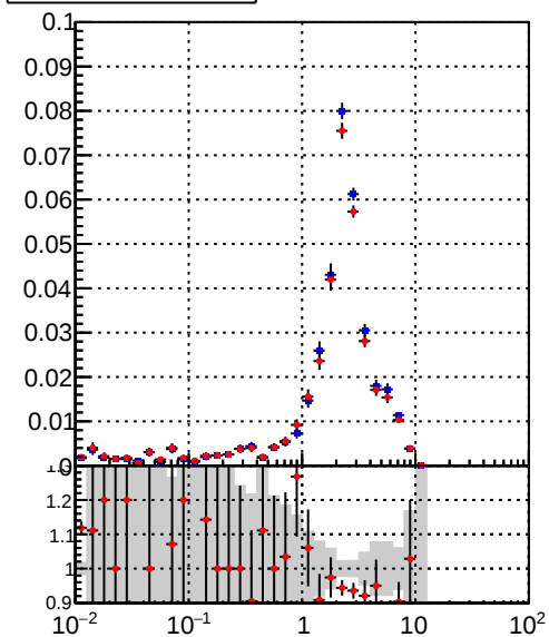
—●— /data2/legianni/BDT-vs-DNN/real-BDT/CMSSW_13_0_0_pre4/src/runrem/DQM_TT_mkFit_ —+— DQM_TT_mkFitRETEST2_
