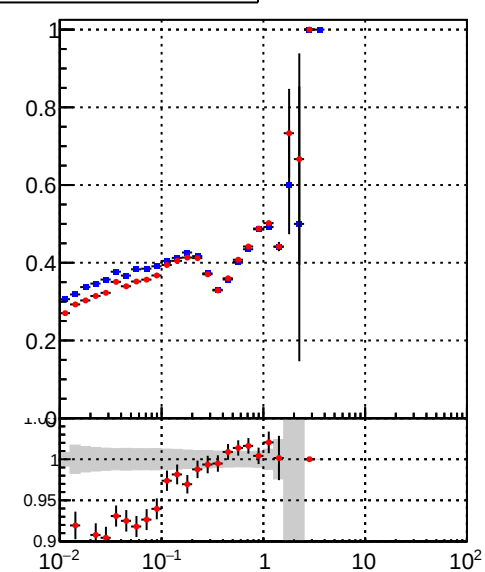
—●— /data2/legianni/BDT-vs-DNN/real-BDT/CMSSW_13_0_0_pre4/src/runrem/DQM_TT_mkFit_ —+— DQM_TT_mkFitRETEST2_
