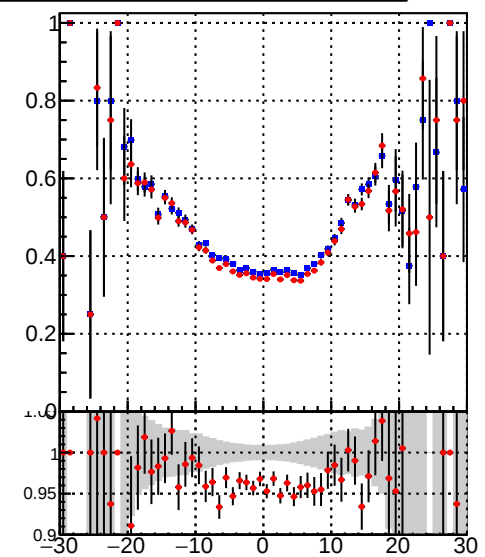
—●— /data2/legianni/BDT-vs-DNN/real-BDT/CMSSW_13_0_0_pre4/src/runrem/DQM_TT_mkFit_ —+— DQM_TT_mkFitRETEST2_
