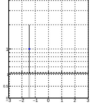
N of associated (recoToSim) tracks vs eta
