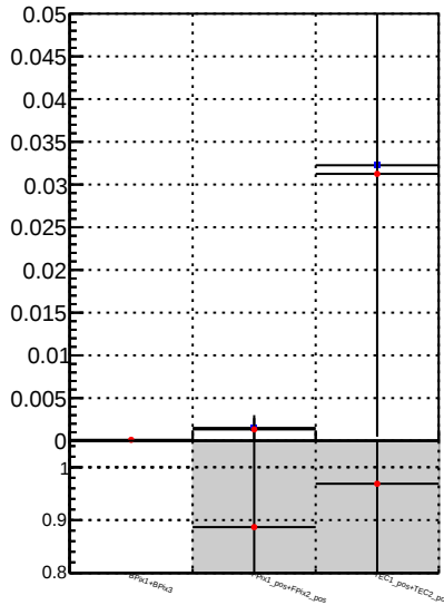
—♦— /data2/legianni/BDT-vs-DNN/real-BDT/CMSSW_13_0_0_pre4/src/runrem/DQM_TT_mkFit_ —★— DQM_TT_mkFitRETEST2
