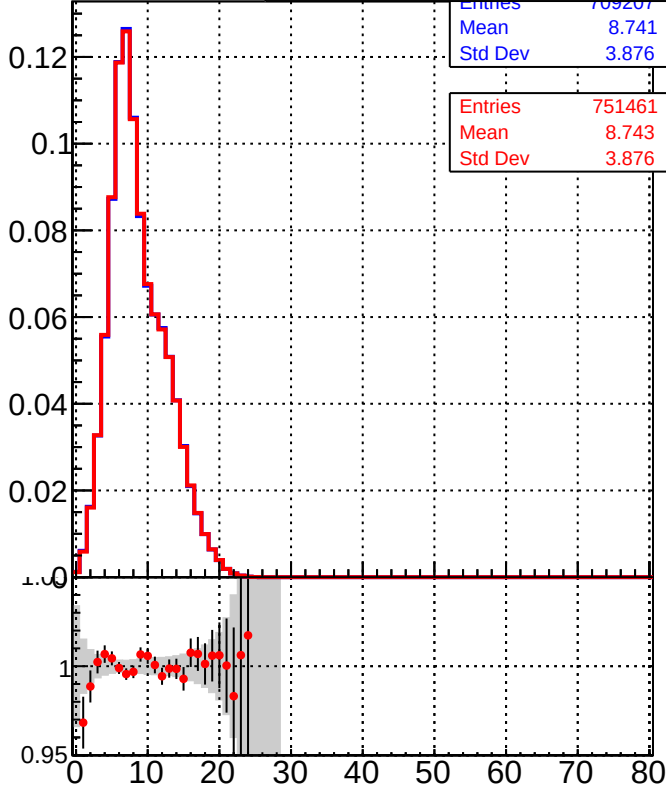
/data2/legianni/BDT-vs-DNN/real-BDT/CMSSW_13_0_0_pre4/src/runrem/DQM_TT_mkFit_ DQM_TT_mkFitRETEST2_
