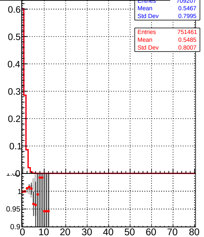
/data2/legianni/BDT-vs-DNN/real-BDT/CMSSW_13_0_0_pre4/src/runrem/DQM_TT_mkFit_ DQM_TT_mkFitRETEST2_
