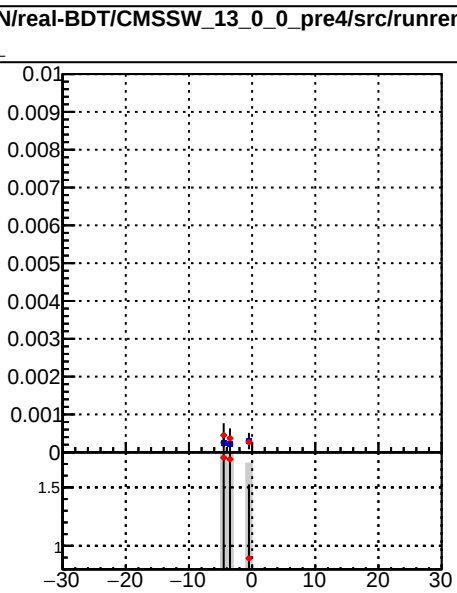
—■— /data2/legianni/BDT-vs-DNN/real-BDT/CMSSW_13_0_0_pre4/src/runrem/DQM_TT_mkFit_ —+— DQM_TT_mkFitRETEST2_ Fake rate vs v
