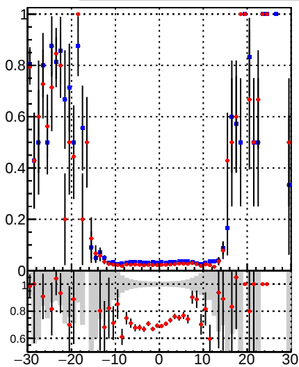
/data2/legianni/BDT-vs-DNN/real-BDT/CMSSW_13_0_0_pre4/src/runrem/DQM_TT_mkFit_ DQM_TT_mkFitRETEST2_ Fake rate vs vertpos
