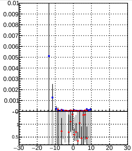
/data2/legianni/BDT-vs-DNN/real-BDT/CMSSW_13_0_0_pre4/src/runrem/DQM_TT_mkFit_ DQM_TT_mkFitRETEST2_ Duplicates Rate vs vertpos
