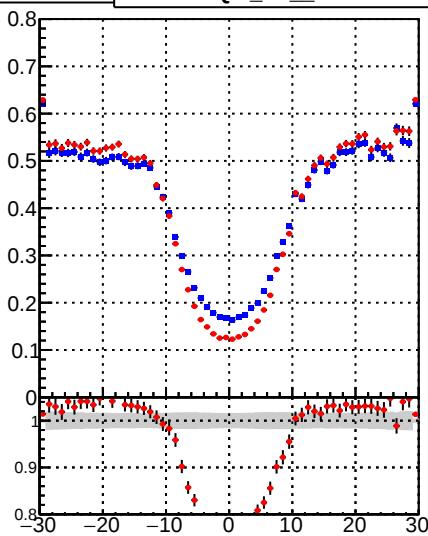
/data2/legianni/BDT-vs-DNN/real-BDT/CMSSW_13_0_0_pre4/src/runrem/DQM_TT_mkFit_ DQM_TT_mkFitRETEST2_ Fake rate vs v
