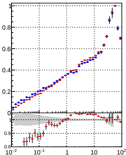
/data2/legianni/BDT-vs-DNN/real-BDT/CMSSW_13_0_0_pre4/src/runrem/DQM_TT_mkFit_ DQM_TT_mkFitRETEST2_ Fake rate vs v
