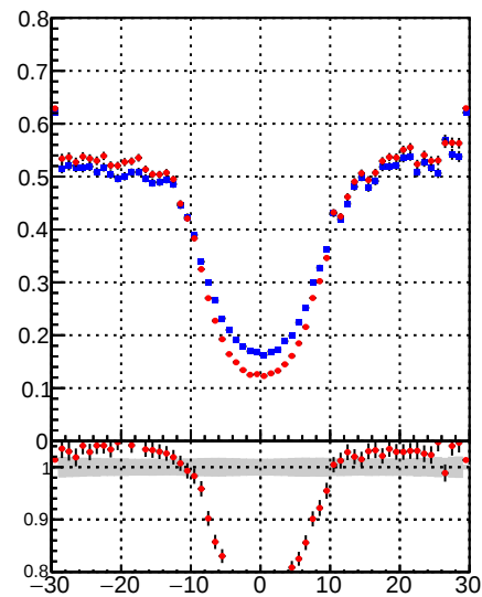
—●— /data2/legianni/BDT-vs-DNN/real-BDT/CMSSW_13_0_0_pre4/src/runrem/DQM_TT_mkFit_ —●— DQM_TT_mkFitRETEST2
