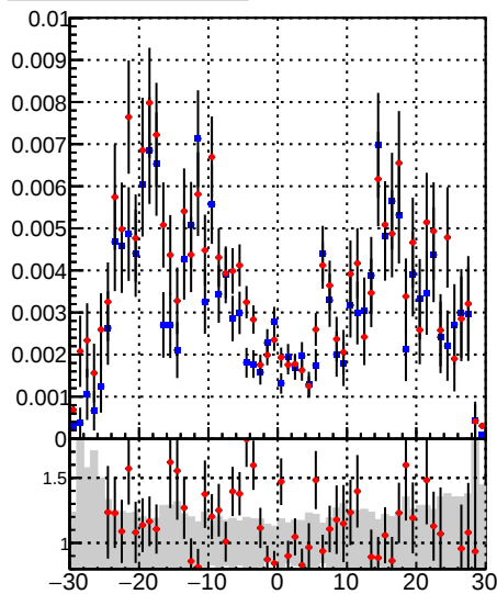
—●— /data2/legianni/BDT-vs-DNN/real-BDT/CMSSW_13_0_0_pre4/src/runrem/DQM_TT_mkFit_ —●— DQM_TT_mkFitRETEST2
