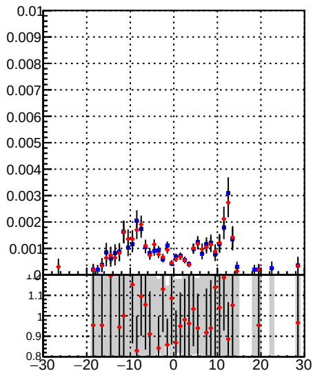
—•— /data2/legianni/BDT-vs-DNN/real-BDT/CMSSW_13_0_0_pre4/src/runrem/DQM_TT_mkFit_ —•— DQM_TT_mkFitRETEST2
