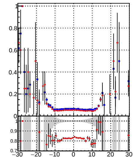
—●— /data2/legianni/BDT-vs-DNN/real-BDT/CMSSW_13_0_0_pre4/src/runrem/DQM_TT_mkFit_ —●— DQM_TT_mkFitRETEST2
