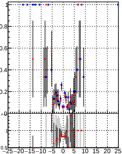
—●— /data2/legianni/BDT-vs-DNN/real-BDT/CMSSW_13_0_0_pre4/src/runrem/DQM_TT_mkFit_ —●— DQM_TT_mkFitRETEST2
