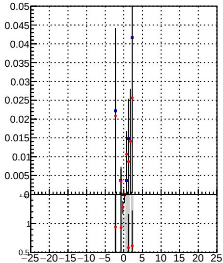
—●— /data2/legianni/BDT-vs-DNN/real-BDT/CMSSW_13_0_0_pre4/src/runrem/DQM_TT_mkFit_ —●— DQM_TT_mkFitRETEST2
