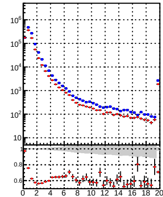
N of reco track vs. \chi^2 for /data2/legianni/BDT-vs-DNN/real-BDT/CMSSW_13_0_0_pre4/src/runrem/DQM_TT_mkFit (blue) and DQM_TT_mkFitRETEST2 (red).
