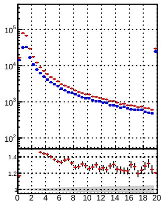
N of reco track vs. \chi^2 for \sqrt{s}=13 TeV, \text{DQM\_TT\_mkFitRETEST2}
