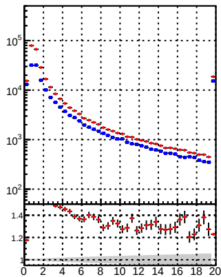
N of reco track vs. \chi^2 for \sqrt{s}=13 TeV, \text{DQM\_TT\_mkFitRETEST2}
