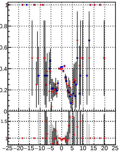
Fake rate vs d — /data2/legianni/BDT-vs-DNN/real-BDT/CMSSW_13_0_0_pre4/src/runrem/DQM_TT_mkFit_ — DQM_TT_mkFitRETEST2_
