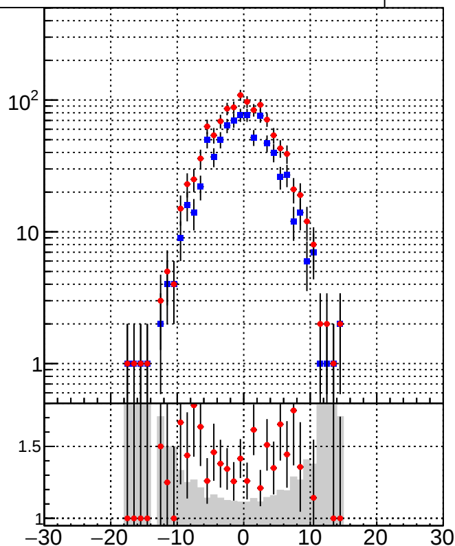
■ /data2/legianni/BDT-vs-DNN/real-BDT/CMSSW_13_0_0_pre4/src/runrem/DQM_TT_mkFit_ ● DQM_TT_mkFitRETEST_
