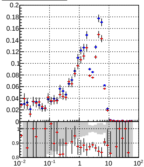
Efficiency vs vertpos Legend: \bullet /data2/legianni/BDT-vs-DNN/real-BDT/CMSSW_13_0_0_pre4/src/runrem/DQM_TT_mkFit_ \bullet DQM_TT_mkFitRETEST_
